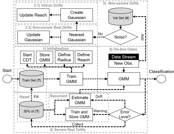
Fig. 2: OGMMF-VRD's overall procedure.
