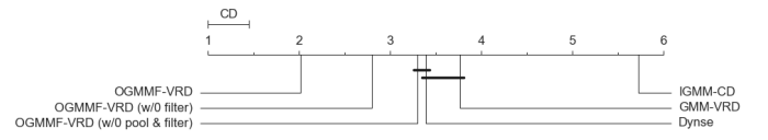
Fig. 7: Friedman ranking for the accuracy obtained in all synthetic datasets with all different noise levels. Friedman's p-value was 9.73E-25 and its ranking is shown from left (best) to right (worst). Any pair of approaches whose distance between them is larger than CD is considered to be different.
