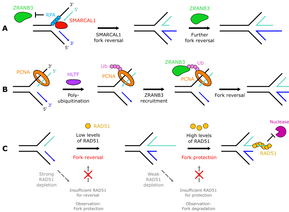
Fig. 2. SNF2-family translocases and RAD51 mediate fork reversal. The translocases SMARCAL1, ZRANB3 and HLF1 may act in a sequential manner. A: SMARCAL1, recruited and stimulated by RPA, may catalyse initial fork reversal. Once RPA has been evicted, ZRANB3 activity will no longer be suppressed, allowing further fork reversal. B: HLF1 polyubiquitinates PCNA, which can recruit ZRANB3 to forks – suggesting ZRANB3 may act downstream of HLF1. C: Differential levels of RAD51 are required for fork reversal versus fork protection. Strong, near complete, RAD51 depletion prevents fork reversal, leading to fork protection. Weaker depletion leaves sufficient RAD51 capable of promoting fork reversal but not enough to support fork protection, leading to degradation by MRE11 and other nucleases.
