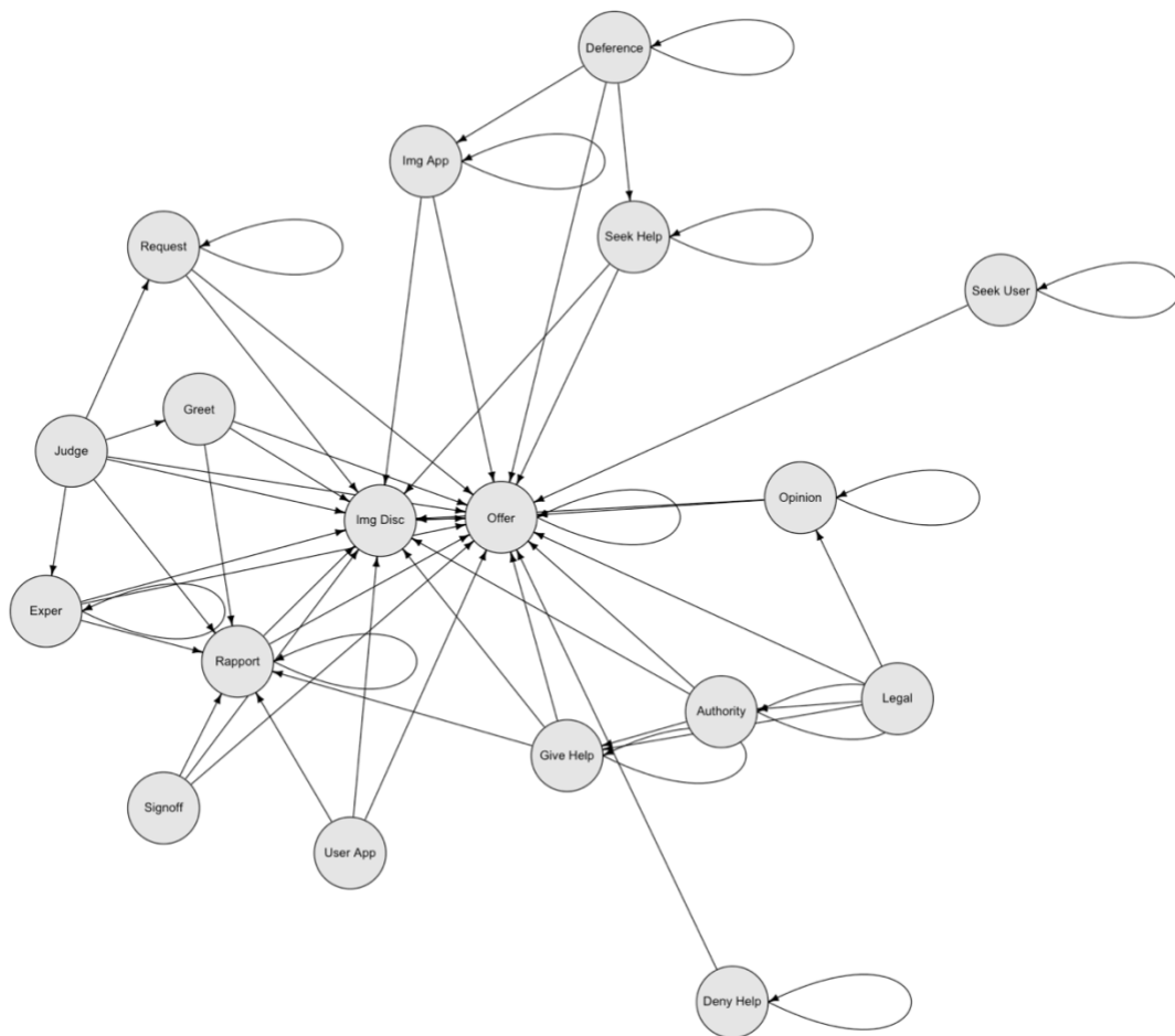
Figure 2. Move transitions of suspected offenders who used the Offering IIOC move.
