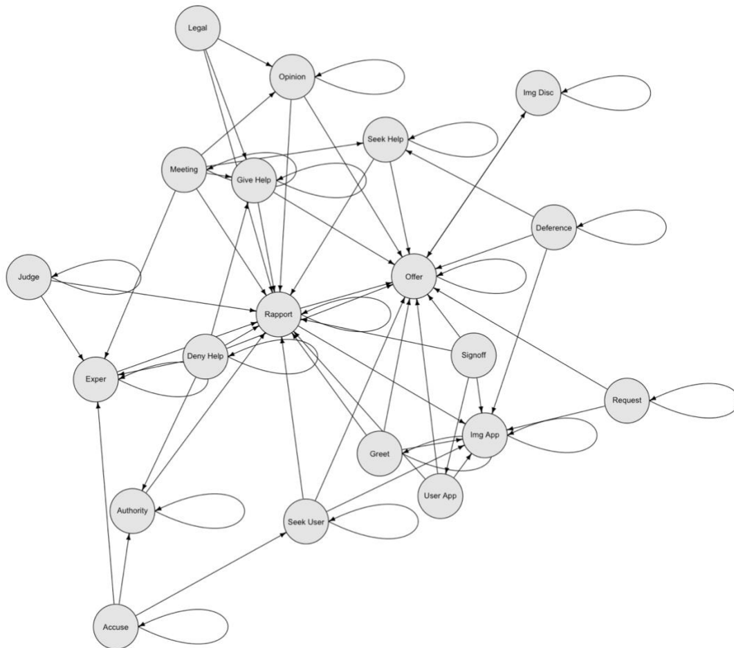
Figure 1. Common move transitions of all users (transition under .10 trimmed).
