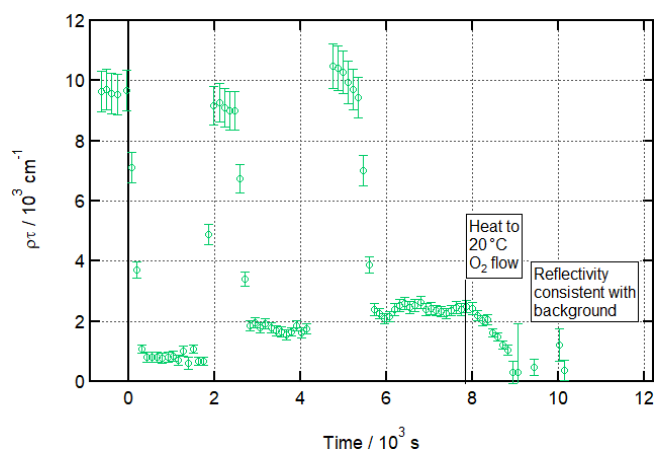
Figure 4. Experiment mimicking an aqueous aerosol droplet exposed to multiple cooking emission peaks and demonstrating the associated build-up of an inert organic film at the air–water interface at low temperatures. Time evolution plot for ozonolysis of 25 \mu\text{L} 1.0 \text{g L}^{-1} d_{34}\text{-OA} ( \text{CHCl}_3 spreading solution) on pure water subphase by 323 \pm 29 ppb \text{O}_3 introduced at t = 0 s and after two additional spreadings of 25 \mu\text{L} 1.0 \text{g L}^{-1} d_{34}\text{-OA} at 3 \pm 1 ^\circ\text{C} .
