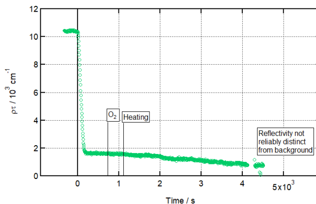
Figure 7. Gradual loss of residue due to increase in temperature. Time evolution plot for ozonolysis of 29\text{ }\mu\text{L} 1.0\text{ g L}^{-1} d_{34} -OA ( \text{CHCl}_3 spreading solution) on pure subphase by 754 \pm 89\text{ ppb} \text{O}_3 introduced at t = 0\text{ s} at 2 \pm 1^\circ\text{C} , with temperature ramping (described in detail in the text) from t = 1035\text{ s} ; error bars are omitted for visual clarity.
