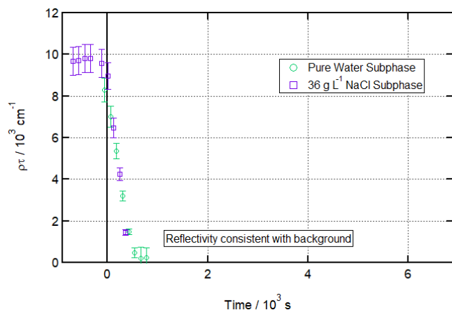
Figure 1. Ozonolysis of an oleic acid monolayer floating on pure vs. salt water. Time evolution plot for ozonolysis of 29\ \mu\text{L}\ 1.0\ \text{g L}^{-1}\ d_{34}\text{-OA} ( \text{CHCl}_3 spreading solution) on pure water (green circles) and 25\ \mu\text{L}\ 1.0\ \text{g L}^{-1}\ d_{34}\text{-OA}\ 36\ \text{g L}^{-1}\ \text{NaCl(aq)} (purple squares) subphases by 323 \pm 29\ \text{ppb}\ \text{O}_3 introduced at t = 0\ \text{s} at 21 \pm 1\ ^\circ\text{C} .
