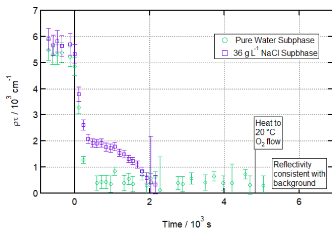
Figure 6. Ozonolysis of a partially deuterated oleic acid monolayer floating on pure vs. salt water. Time evolution plot for ozonolysis of 17 \mu\text{L} 1.3 \text{g L}^{-1} d_{18} -OA ( \text{CHCl}_3 spreading solution) on pure water (green circles) and 36 \text{g L}^{-1} \text{NaCl(aq)} (purple squares) subphases by 323 \pm 29 ppb \text{O}_3 introduced at t = 0 s at 3 \pm 1^\circ\text{C} (pure water) or -2 \pm 1^\circ\text{C} (salt water).
