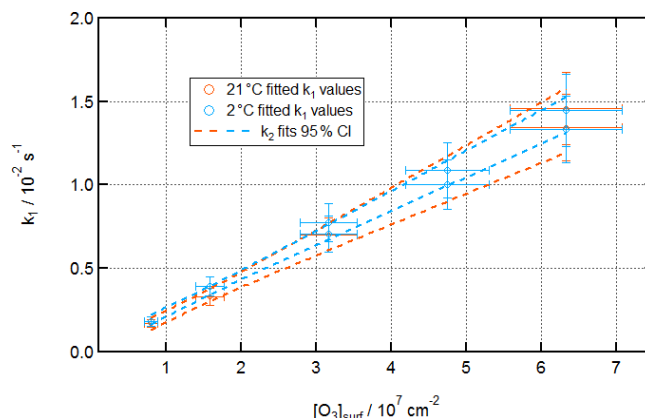
Figure 8. Kinetics of ozonolysis of the oleic acid monolayer on pure water at room and low temperatures. Fitted k_1 pseudo-first-order rate constants against [O_3]_{\text{surf}} at 21 \pm 1 °C (orange) and 2 \pm 1 °C (aqua).
