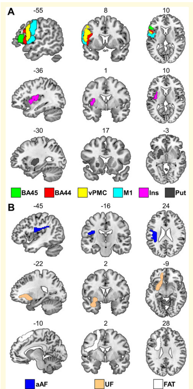
Figure 1 The nine atlas-defined regions of interest. (A) The top three rows show the six left cortical and subcortical grey matter regions defined using the Brainnetome atlas (Fan et al., 2016). (B) The bottom three rows show the three white matter tracts defined using tractography-based atlases of human brain connections (Catani and Thiebaut de Schotten, 2008; Thiebaut de Schotten et al., 2011; Rojkova et al., 2016). FAT = frontal aslant tract; Ins = superior central insula; Put = putamen; UF = uncinate fasciculus.
