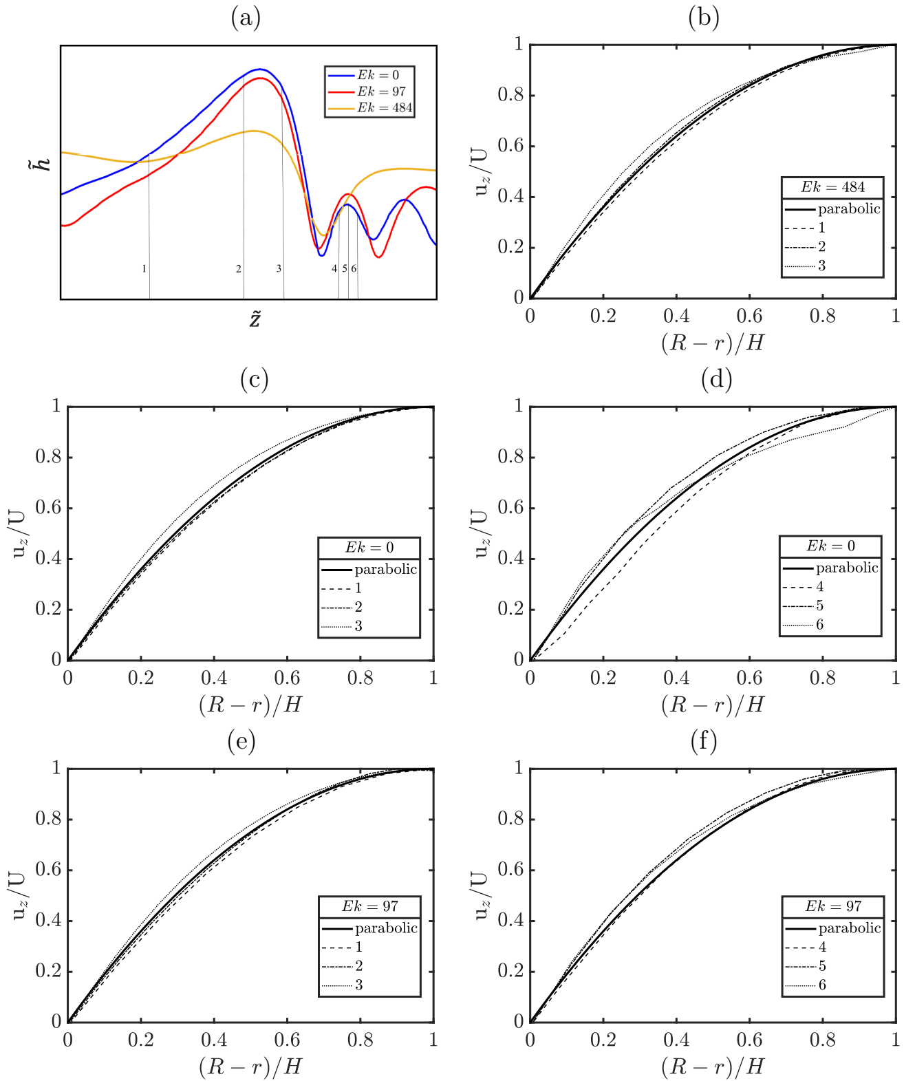
FIG. 4: Velocity profiles in the film underneath the solitary waves for various Ek with the rest of the parameters remaining unaltered from Fig. 2: (a) three interfacial profiles for Ek = 0 , 97, and 484, with the points ‘1’-‘6’ marking the locations at which the radial variation of the axial velocity component normalised by its maximal value, u_z/U , is plotted in (b), (c) and (d), and (e) and (f) for Ek = 484 , 0, and 97, respectively; also shown in (b)-(f) is a parabolic profile for reference. The radial coordinate is normalised by the local maximum film height H
