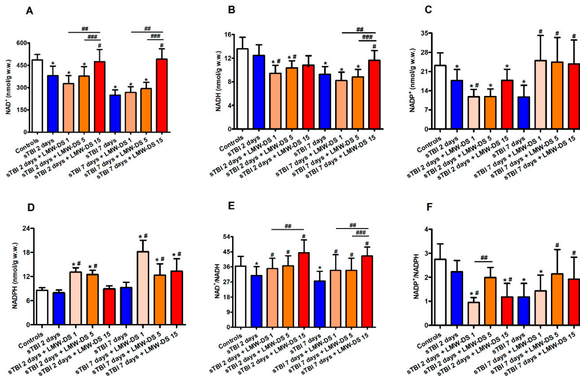
Figure 5. Effect of subcutaneous injection of increasing doses of LMW-DS (ILB®) on the cerebral concentrations of \text{NAD}^+ (A), \text{NADH} (B), \text{NADP}^+ (C), and \text{NADPH} (D), and of the \text{NAD}^+/\text{NADH} (E) and \text{NADP}^+/\text{NADPH} (F) ratios as valuable indicators of oxido-reductive metabolism of the nervous cell energy state. The parameters of interest were determined by HPLC on deproteinized cerebral homogenates at 2 and 7 days post-impact, both in untreated sTBI rats (TBI 2 days and TBI 7 days) and in rats receiving 1, 5, or 15 mg/kg b.w. LMW-DS (ILB®) administered 30 min after sTBI. Controls are represented by sham-operated rats. Values are the mean \pm SD of 12 different animals and are expressed as nmol/g w.w. * Significantly different from sham-operated control rats, p < 0.05 . # Significantly different from the corresponding time point of untreated sTBI rats, p < 0.05 . ## Significantly different from LMW-DS 1, p < 0.05 . ### Significantly different from LMW-DS 5, p < 0.05 .
