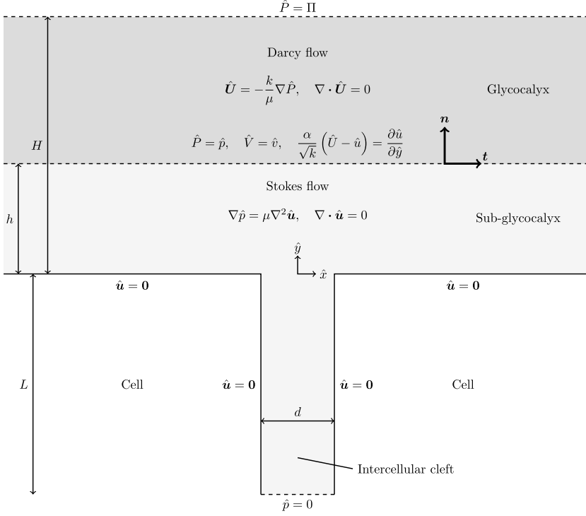
FIG. 8. Schematic of the dimensional flow problem with a sub-glycocalyx. We consider a two-dimensional setup, with the impermeable sub-glycocalyx and intercellular cleft walls representing the endothelial cells. Darcy flow governs the dark gray region, Stokes flow governs the light gray region, and the white regions denote the impermeable endothelial cells.
