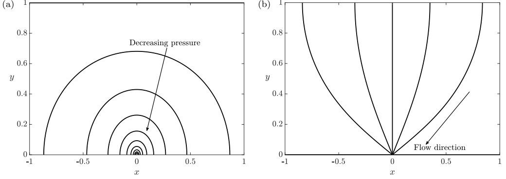
FIG. 6. (a) A pressure contour map in Region I from P = 0.55 to P = 1 in increments of 0.05, as given by (14). (b) The streamlines in Region I, as given by the complex conjugate of (14). We use \kappa = 0.3 for both panels.
